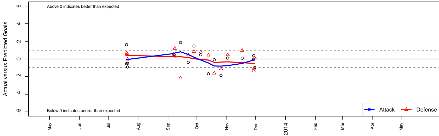
IE Surf G99 Dots are actual minus expected GF (blue circles) and GA (red triangles). Blue line is smoothed change in attack strength. Red is smoothed change in defense strength.
